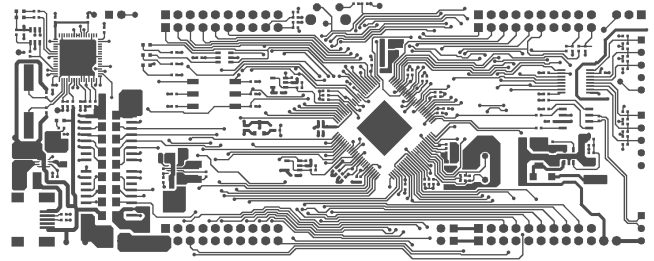
Figure 9. Top Copper
