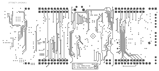
Figure 13. Bottom Copper
