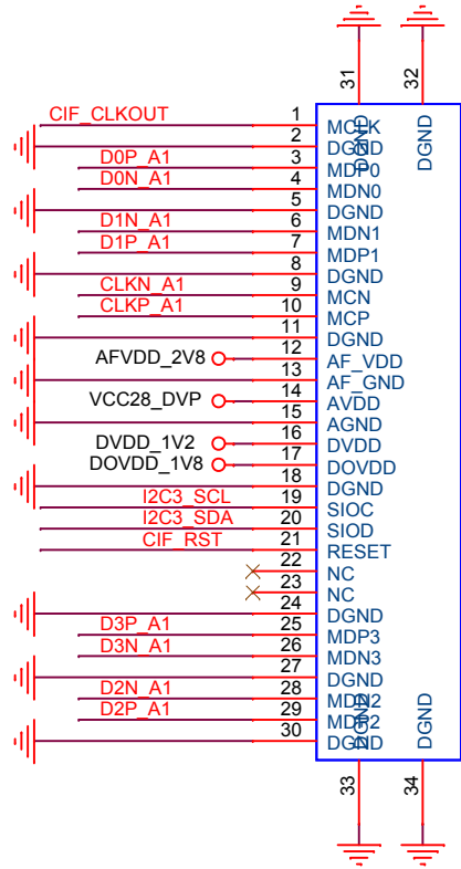
J23 OV13850
