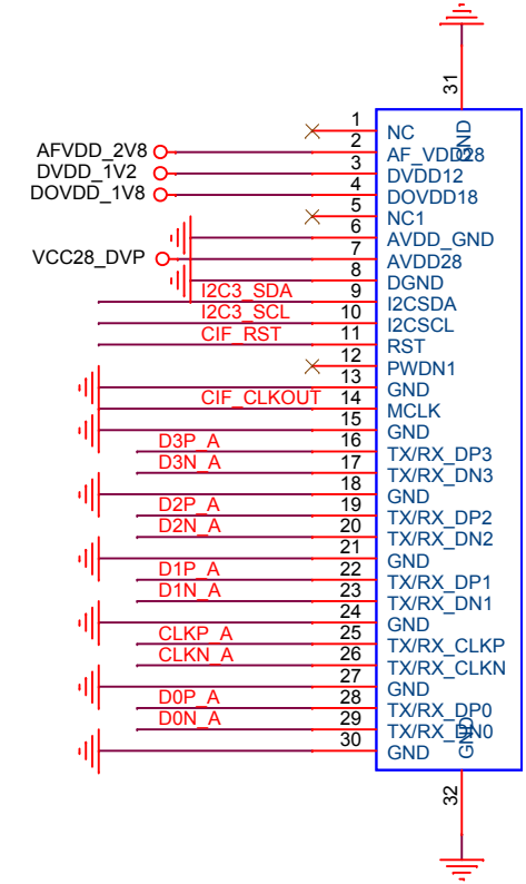
J30 CON30PIN_0D5MM
