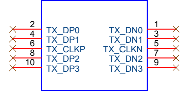
J80 SIP_10PIN_2.54MM
